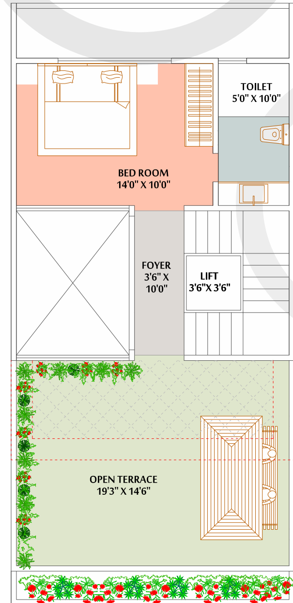
2nd Floor Plan (Alt-07)
